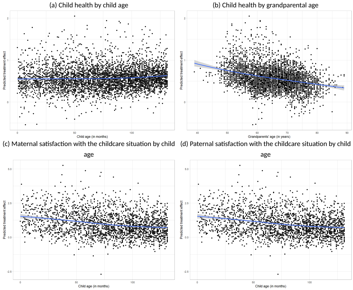
Figure C.3: Causal forest predictions
