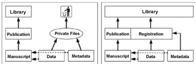
Figure 1. The traditional publication method for datasets on the left, a possible new structure on the right
