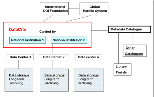
Figure 3. The overall structure of DataCite
