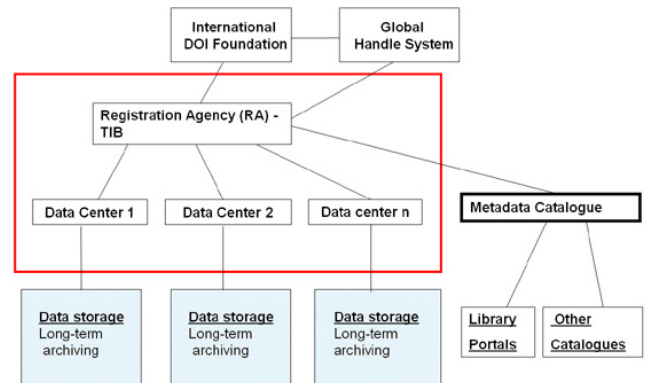
Figure 2. The overall structure of TIB's DOI Registration Agency
