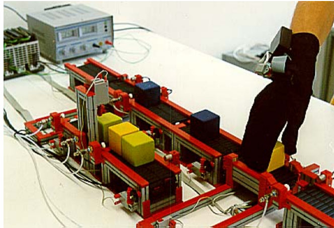
Fig. 2: Driving a real Model with a PLC
