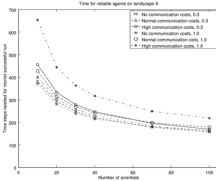
Figure 7: Time Steps Needed for Successful Runs (Monist Criterion) with Reliable Agents and Different Communication Costs
