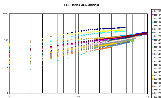
Figure 2: Bradford graphs (log-log plot) for 25 topics from the CLEF evaluation 2005. Journals are on the x-axis, journal articles are cumulated on the y-axis. Documents mean: 142, Journals total mean: 61, core mean: 4.64, z2 mean: 17.24, z3 mean: 39.56.
