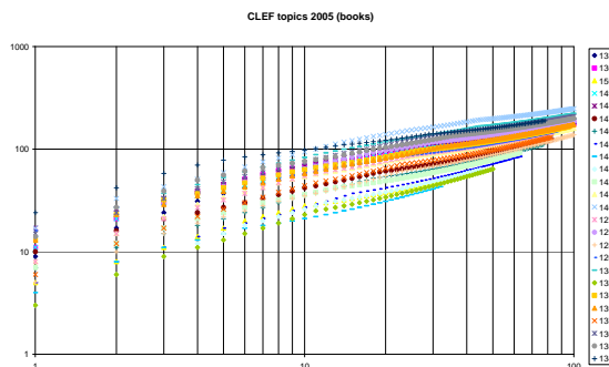
Figure 3: Bradford graphs (log-log plot) for the same 25 topics from the 2005 sample. Publishers are on the x-axis, monographs are cumulated on the y-axis. Documents mean: 211, Publishers total mean: 90, core mean: 8.60, z2 mean: 29.56, z3 mean: 51.88.
