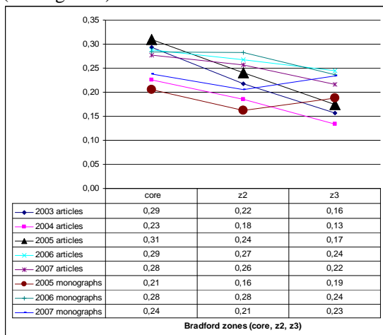
Figure 4: Precision values for items (articles and monographs) in core, z2 and z3 (125 topics from the CLEF evaluation, compare Table 2). The both data sets CLEF 2005 journal articles and monographs (documents in Figure 2 and 3) are displayed with larger data points.
