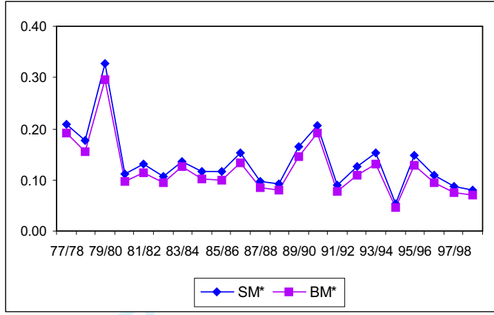
Figure A2: Regional mobility measured by SM^*(\Pi, \rho) and BM^*(\Pi, \rho) , m = 8 .
