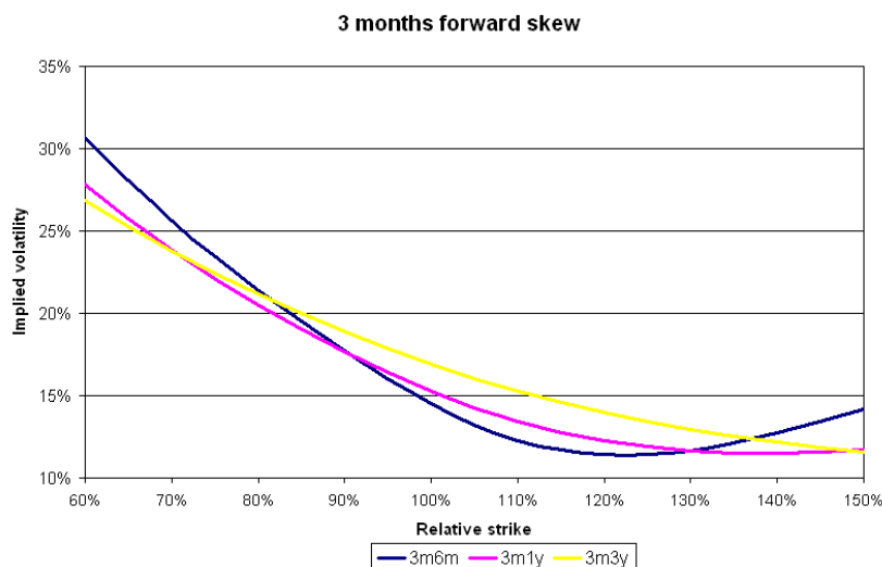
FIGURE 7. Implied forward volatility skews 3 months from now. For example the code 3m1y means that T' equals 3 months and that the expiry T can be calculated as T = (T' + 1) year, where T', T are as defined in subsection B.3. Along the line of abscisse we plot the forward strike \alpha (i.e. the “moneyness” of the ordinary call option that the forward-start becomes at time T' ) as defined in formula (17). The ordinate axis contains the forward volatility values expressed in percentage, as implied by the model.
