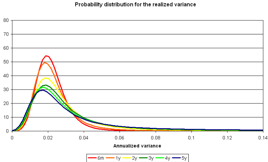
FIGURE 11. Probability distribution functions for the realized variance, quoted in annual terms, for maturities between 6 months and 5 years as given by our model after calibration to the implied volatility surface of the S&P 500 (see section 4 for details). These pdfs are marginal distributions obtained from the joint probability distribution function (6) by integrating it in the dimension of the spot value of the index.
