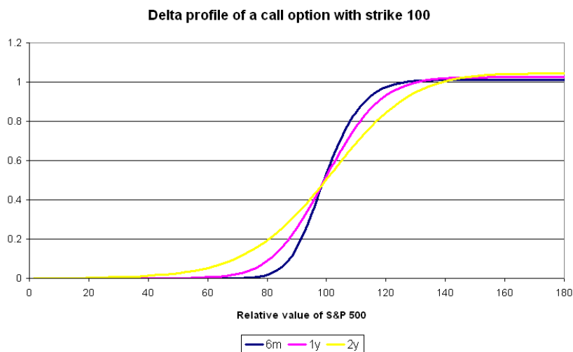
FIGURE 4. Delta profiles of call options on the S&P 500 with maturities between 6 months and 2 years, all struck at 100. We calculate the delta of a call option (i.e. \Delta(S) = \frac{\partial C}{\partial S}(S) ) for all lattice points S using a symmetric difference as described in subsection 5.1 Notice that we are using the underlying index S and the strike of the options on their relative scales with respect to the level at which the index was trading when the snapshot of the market was taken.
