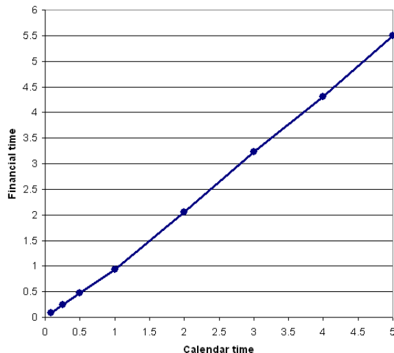
FIGURE 3. Deterministic time-change f(t) (measured in years) as a function of calendar time t (also in years). Function f was used in the calibration of the model to the vanilla surface of the S&P 500.
