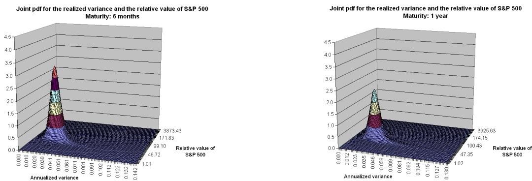
FIGURE 15. Joint probability distribution function for the annualized realized variance and the spot rate of S&P 500 in 6 months' and 1 year's time.
