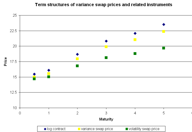
FIGURE 18. Term structures of variance swap prices for maturities between 6 months and 5 years as implied by the vanilla market data using the calibrated model (for precise values see table 3). The delivery prices (i.e. fair strikes) are computed as \mathbb{E}_0[\Sigma_T] , where \Sigma_T is the annualized realized variance for each tenor T . Everything is expressed in terms of volatility, i.e. the prices are in percent and are obtained by taking the square root of the variance. We also plot fair delivery prices for volatility swaps. The convexity bias implied by the model can be clearly observed. The value of the log contract, defined in equation (20), given by the underlying model is also plotted. Observe that this portfolio of options is always worth more than the corresponding variance swap because, in our model, we only allow for down jumps (see section 4). This behaviour is exactly as predicted by the analysis in (Demeterfi et al. 1999b) (equation 42) when they added a single down-jump to the underlying process and studied its influence on the static hedge (20) for the variance swap.
