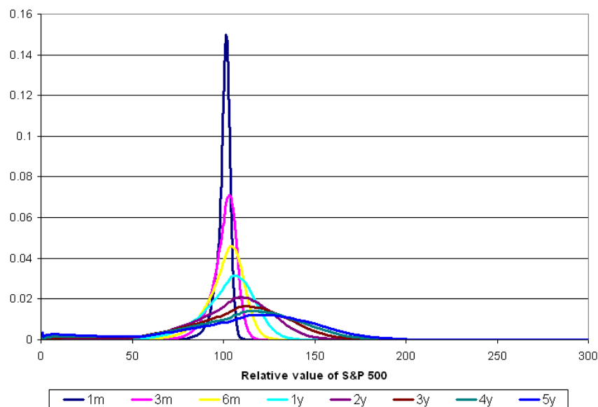
FIGURE 2. Implied probability density function for the S&P 500 under the forward measure. The value of the S&P 500 plotted along the line of abscisse is a relative value (in percent) with respect to the current level of spot. The pdfs between 6 months and 5 years can also be viewed as the rescaled marginals of the joint pdfs in figures 15, 16, and 17.
