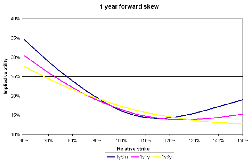
FIGURE 9. Implied forward volatility skews 1 year from now. For example the code 1y6m means that T' equals 1 year and that the expiry T can be calculated as T = (T' + 6 \text{ months}) , where T', T are as defined in subsection B.3. Along the line of abscisse we plot the forward strike \alpha (i.e. the “moneyness” of the ordinary call option that the forward-start becomes at time T' ) as defined in formula (17). The ordinate axis contains the forward volatility values expressed in percentage, as implied by the model.
