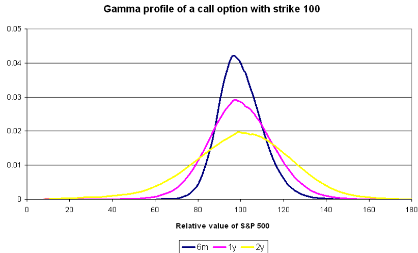
FIGURE 5. Gamma profiles of call options on the S&P 500 with maturities between 6 months and 2 years, all struck at 100. We calculate the gamma of a call option (i.e. \Gamma(S) = \frac{\partial^2 C}{\partial S^2}(S) ) for all lattice points S using a symmetric difference as described in subsection 5.1. The same comment as in figure 4, about the relative value of the index and the strike, applies.
