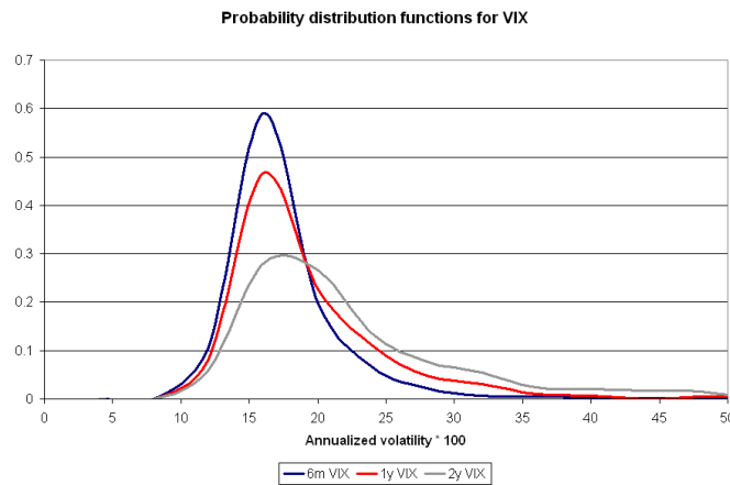
FIGURE 19. Probability distribution functions of the implied volatility index for maturities between 6 months and 2 years.
