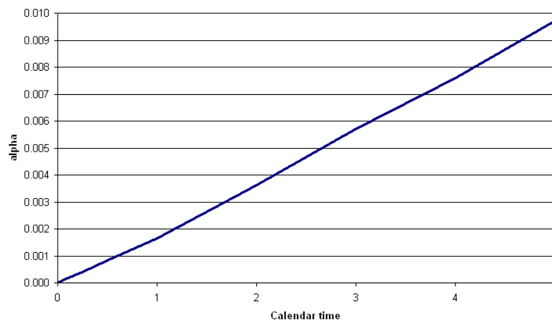
Spacing of the grid for the realized variance
