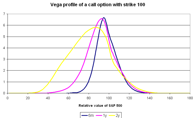
FIGURE 6. Vega profiles of call options on the S&P 500 with maturities between 6 months and 2 years, all struck at 100. We are calculating the vega of a call option by bumping the current volatility regime, repricing the option and plotting the difference from the original option value, for all points on the lattice. Notice that vega and gamma profiles are very similar in shape but different in magnitude, which is consistent with the general market view on the two Greeks.
