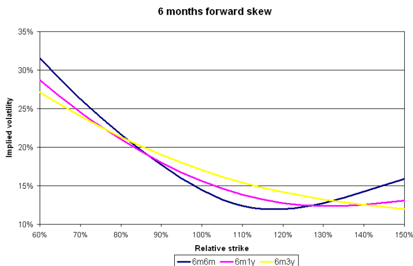
FIGURE 8. Implied forward volatility skews 6 months from now. For example the code 6m1y means that T' equals 6 months and that the expiry T can be calculated as T = (T' + 1) year, where T', T are as defined in subsection B.3. Along the line of abscisse we plot the forward strike \alpha (i.e. the “moneyness” of the ordinary call option that the forward-start becomes at time T' ) as defined in formula (17). The ordinate axis contains the forward volatility values expressed in percentage, as implied by the model.
