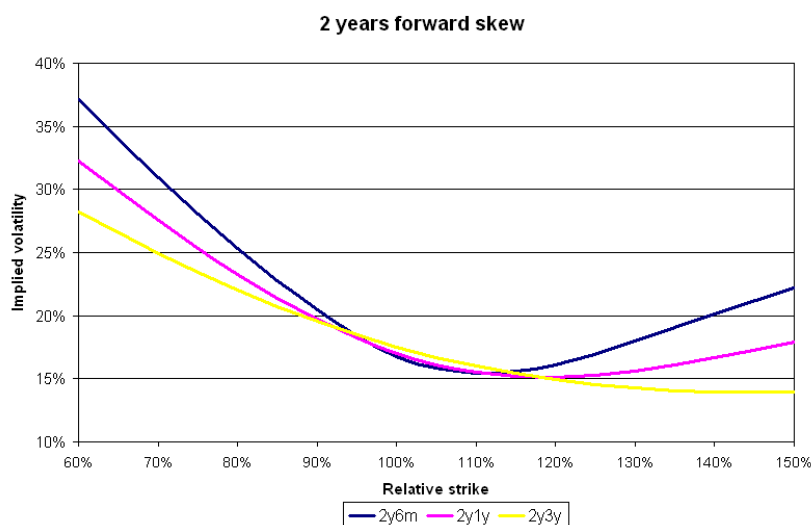
FIGURE 10. Implied forward volatility skews 2 years from now. For example the code 2y6m means that T' equals 2 years and that the expiry T can be calculated as T = (T' + 6 \text{ months}) , where T', T are as defined in subsection B.3. Along the line of abscisse we plot the forward strike \alpha (i.e. the “moneyness” of the ordinary call option that the forward-start becomes at time T' ) as defined in formula (17). The ordinate axis contains the forward volatility values expressed in percentage, as implied by the model.
