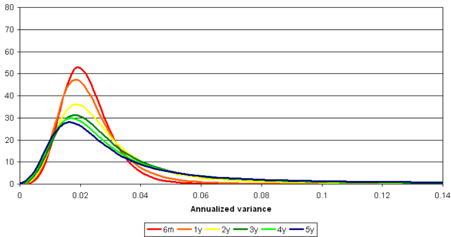
FIGURE 13. Probability distribution functions for the realized variance, quoted in annual terms, for maturities between 6 months and 5 years as given by the model used in figure 11, but with zero jump intensities, based on two volatility regimes. The model parameters are the same as the ones given in table 1 of section 4 but with \nu_{\alpha}^{-} = 0 , for \alpha = 0, 1 .
