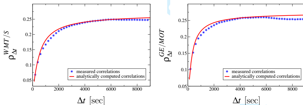
Figure 9: The measured and the analytically computed cross-correlation coefficients as a function of sampling time scale for the pairs WMT/S and GE/MOT. Details on the goodness parameter of the measured and computed correlations can be found in Table 2.
