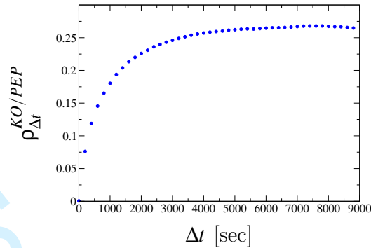
Figure 1: The cross-correlation coefficient as a function of sampling time scale for the period 1993–2003 for the Coca-Cola Pepsi pair. Several hours are needed for the correlation to reach its asymptotic value.
