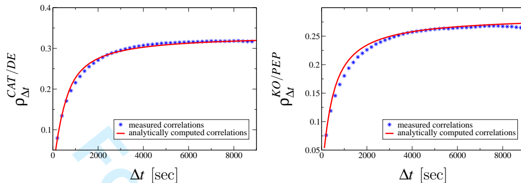
Figure 8: The measured and the analytically computed cross-correlation coefficients as a function of sampling time scale for the pairs CAT/DE and KO/PEP. Note that using only the autocorrelations and cross-correlations measured on the smallest time scale ( \Delta t_0 = 120 seconds) we are able to give reasonable fits to the cross-correlations on all time scales. Details on the goodness parameter of the measured and computed correlations can be found in Table 2.
