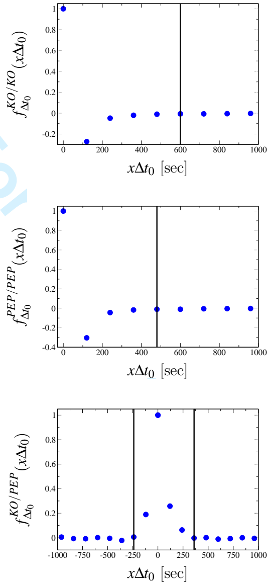
Figure 7: Top: The decay of lagged autocorrelations for KO. Middle: The decay of lagged autocorrelations for PEP. Bottom: The decay of lagged cross-correlations for KO/PEP pair. A vertical lines show the threshold up to which we take the decays into account, for larger lags we assume them to be zero. Sampling time scale is \Delta t_0 = 120 seconds on all three plots.
