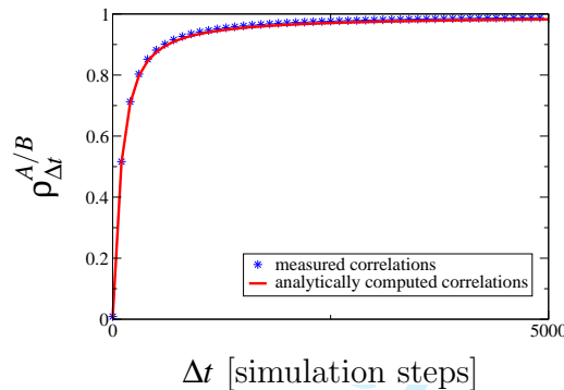
Figure 6: The measured and the computed cross-correlation coefficients using exponential decay function as a function of sampling time scale for the simulated time series with exponentially distributed waiting times. The analytic fit is in very good agreement with the Epps curve.
