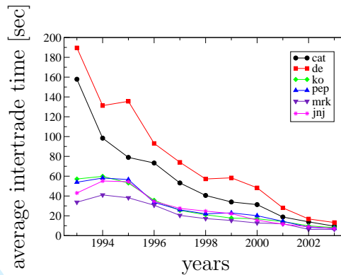
Figure 4: The average intertrade time for the years 1993 to 2003 for some example stocks (CAT, DE, KO, PEP, MRK, JNJ). The activity was growing almost monotonically.
