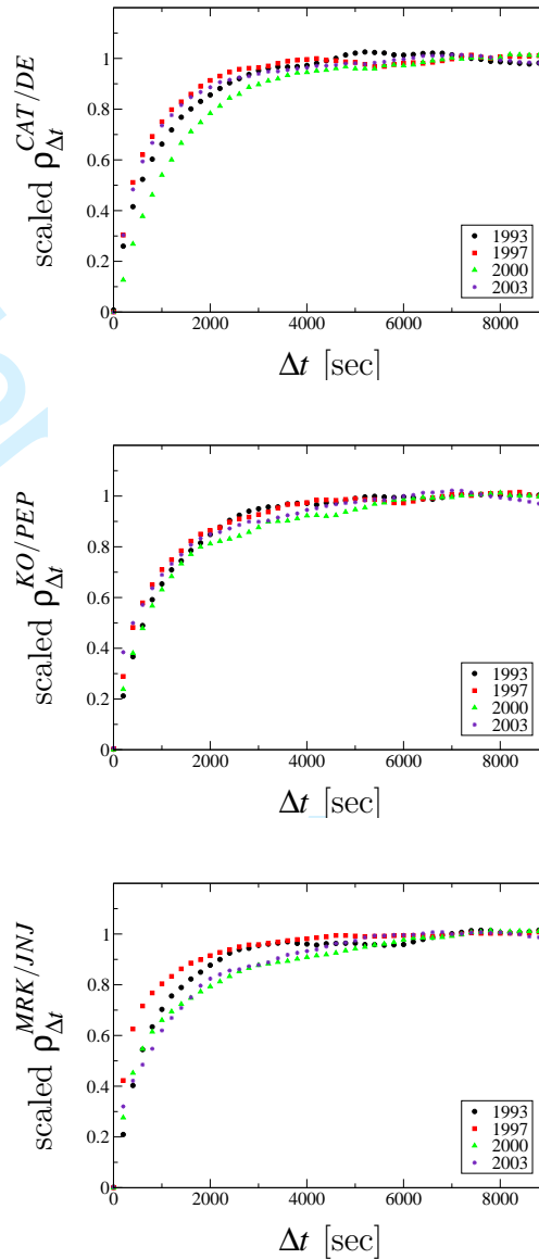
Figure 3: The Epps curves scaled with the asymptotic cross-correlation values for the CAT/DE (top), KO/PEP (middle) and MRK/JNJ (bottom) pairs for the years 1993, 1997, 2000 and 2003. The scaled curves give a reasonable data collapse in spite of the considerably changing trading frequency, showing that the characteristic time of the Epps effect does not change with growing activity.
