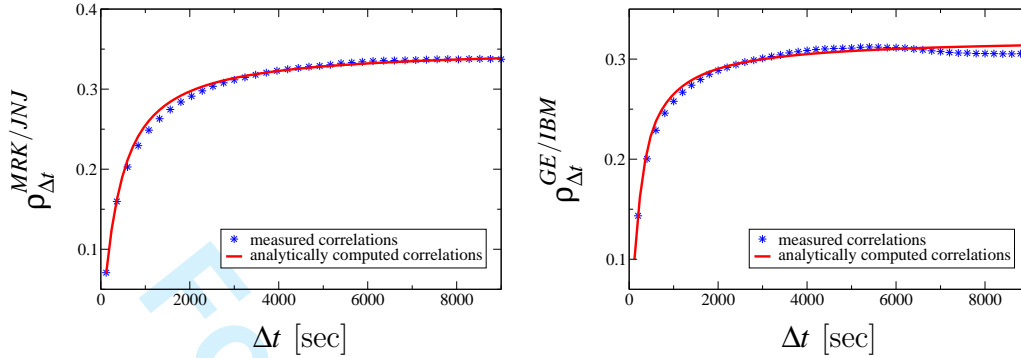
Figure 10: The measured and the analytically computed cross-correlation coefficients as a function of sampling time scale for the pairs MRK/JNJ and GE /IBM. Details on the goodness parameter of the measured and computed correlations can be found in Table 2.
