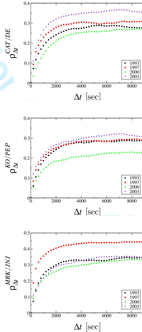
Figure 2: The Epps curves for the CAT/DE (top), KO/PEP (middle) and MRK/JNJ (bottom) pairs for the years 1993, 1997, 2000 and 2003. The asymptotic value of the cross-correlations varies in time.
