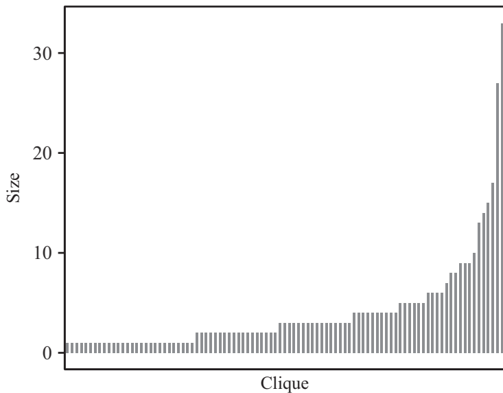
FIGURE 4. Distribution of clique size.
