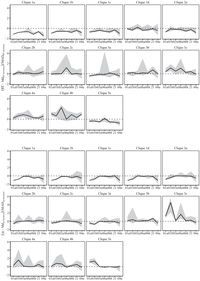
FIGURE 5. Centered trajectories of median and middle 50% ranges of time spent on task in seconds (upper panel) and number of performed actions (lower panel) across all items of PSI of the PIAAC PSTRE domain for the 13 most dominant incorrect behavioral pattern groups on Item U01a. The items shown on the horizontal axis are ordered by item positions.
