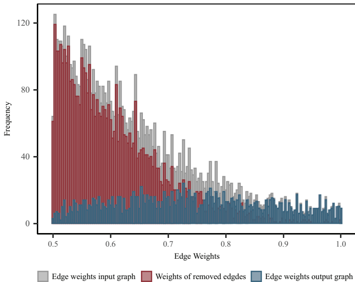
FIGURE 3. Distribution of edge weights of the input and output graphs as well of weights of edges removed in the cluster edge deletion procedure.
