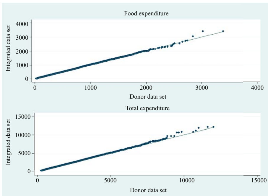
Fig. 6. Q-Q plot of food expenditure and total expenditure.
