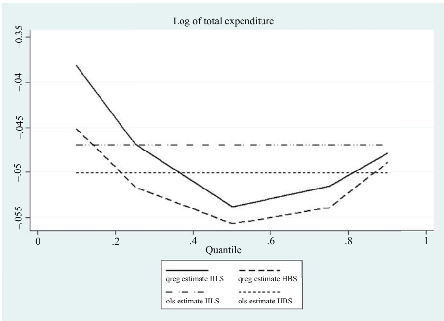
Fig. 11. Estimated coefficient of total expenditure with OLS regression and quantile regression.
