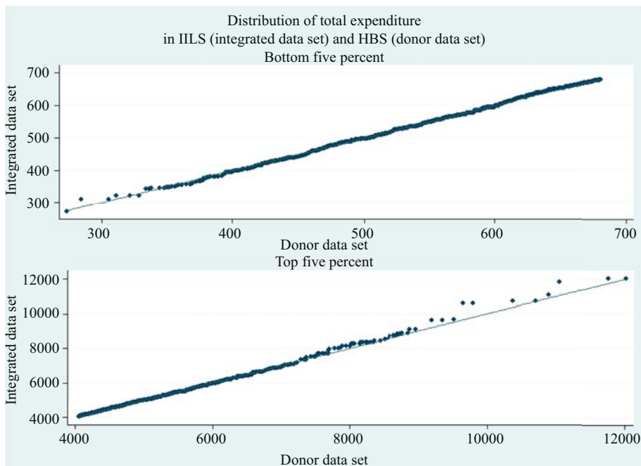
Fig. 8. Q-Q plot of total expenditure: focus on the tails.
