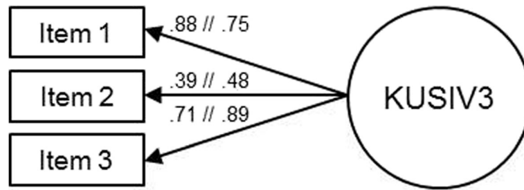
Fig. 1 Unidimensional measurement model of KUSIV3 with standardized coefficients. The negatively keyed item is reverse-scored. The coefficients of the German sample are presented after the double slash. Item error terms are omitted for clarity. N_{UK} = 468 ; N_{DE} = 474
