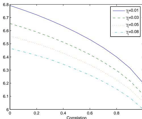
Figure 4: Implied bond yield, varying \gamma_i
