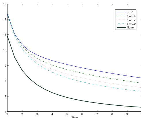
Figure 2: Implied yield curve, \omega_1 = 0.5
