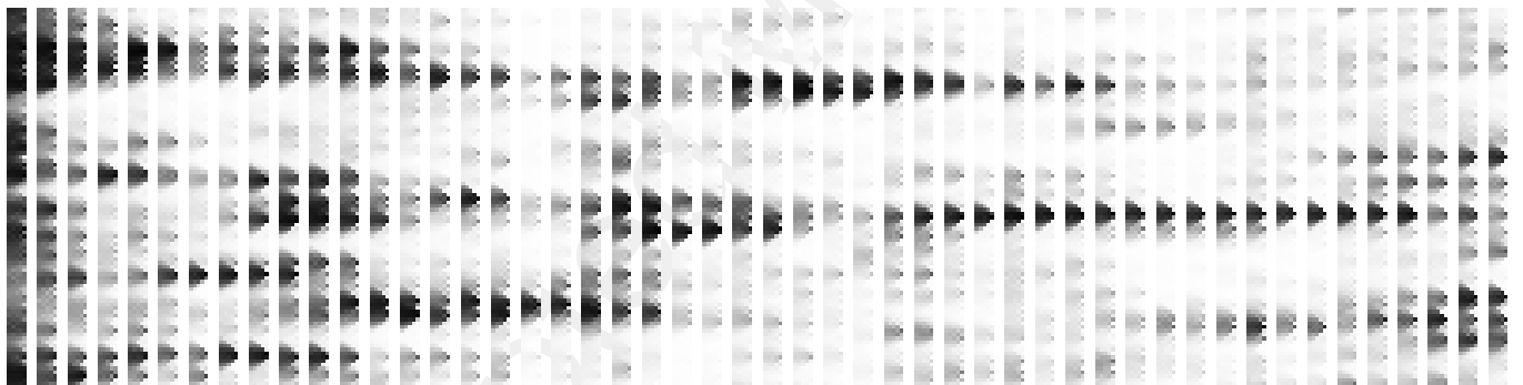
Figure 7: Successive patterns of wealth from left (at time 200) to right (at time 10000). These patterns are rotated by 90 degrees with respect to their orientation in figures 5 and 6. Input layer is the left layer of each pattern. Following the horizontal axis we see that patterns are metastable, with life times of the order of a few thousands (parameter set-up: time lag = 1, 100x5 lattice).
