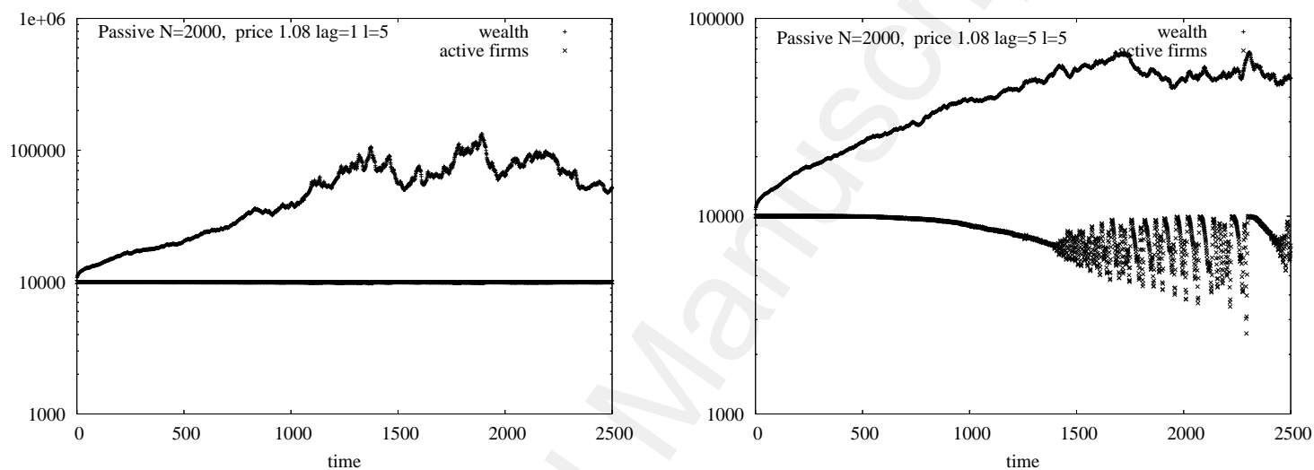
Figure 2: Time evolution of total wealth ( '+' ) and number of active firms ( 'x' ). The network has 5 layers, 2000 firms per layer, \mathcal{P} = 0.05 (the failure probability). The left diagram corresponds to a small time lag equal to 1. between bankruptcy and firm re-birth, the right one to a larger time lag equal to 5. Vertical scale is logarithmic. The large wealth fluctuations do not correlate with avalanches of bankruptcies when they occur.
